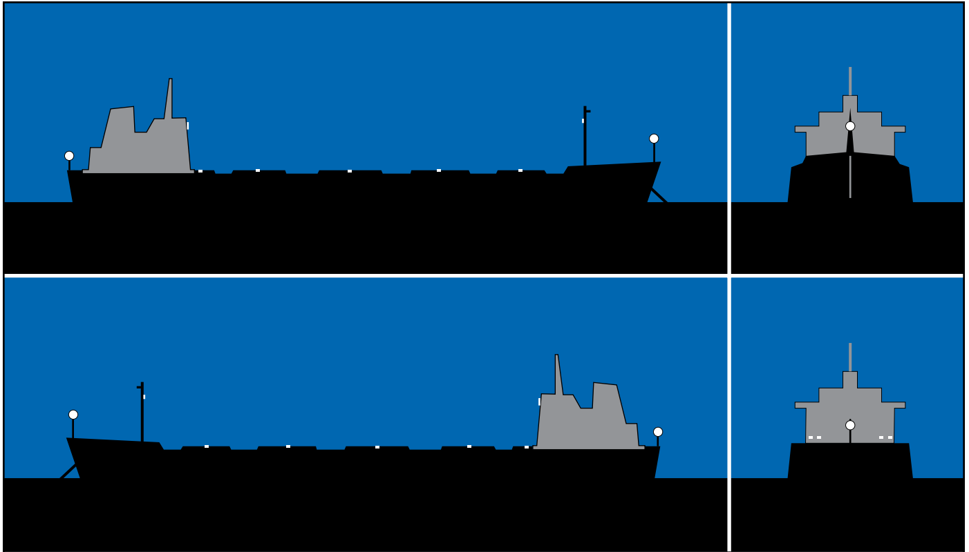
Vessel at anchor, probably 100 metres or more in length. Must have illuminated deck lights.
