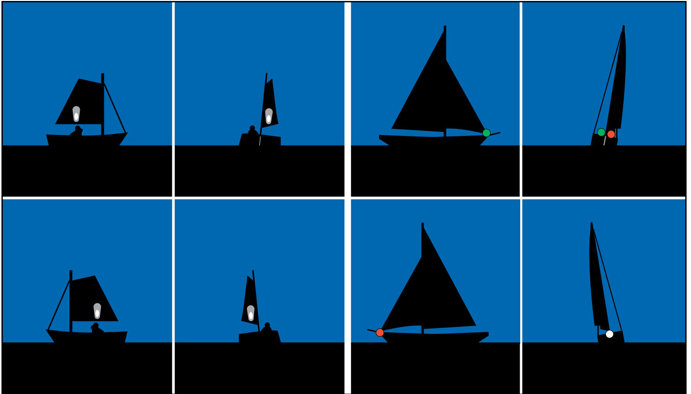
Left set / Sailing vessel under way, less than 7 metres in length. Right set / Sailing vessel under way.
