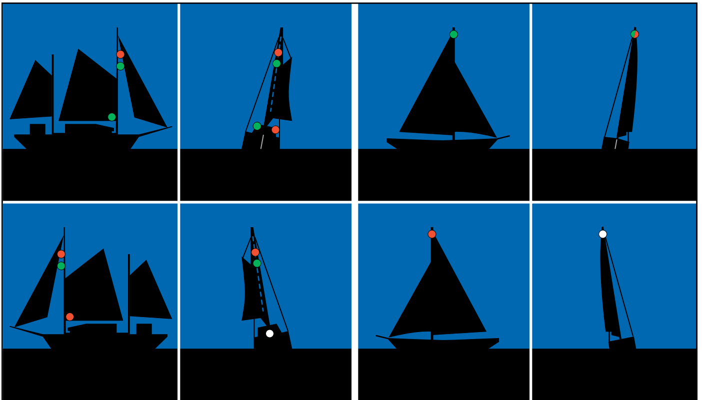
Left set / Sailing vessel under way, with optional lights. Right set / Sailing vessel under way, less than 20 metres in length.
